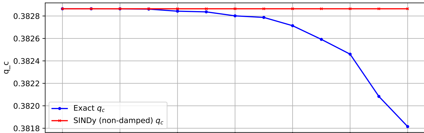
Trajectory 299 (non-damped)
