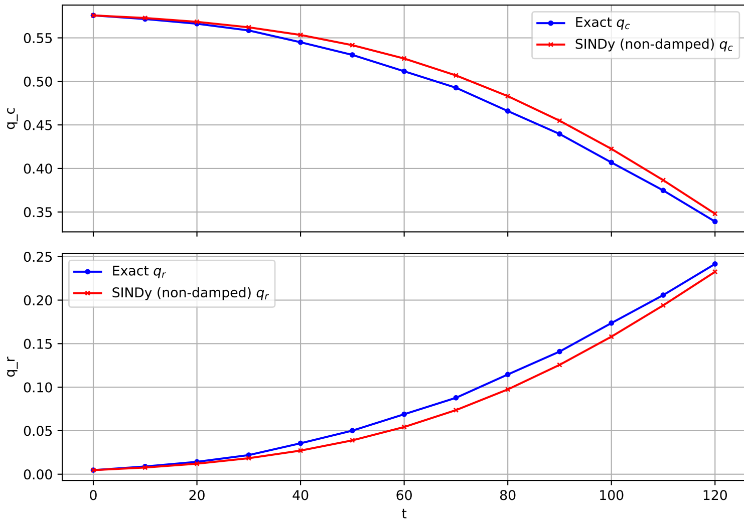
Trajectory 309 (non-damped)
