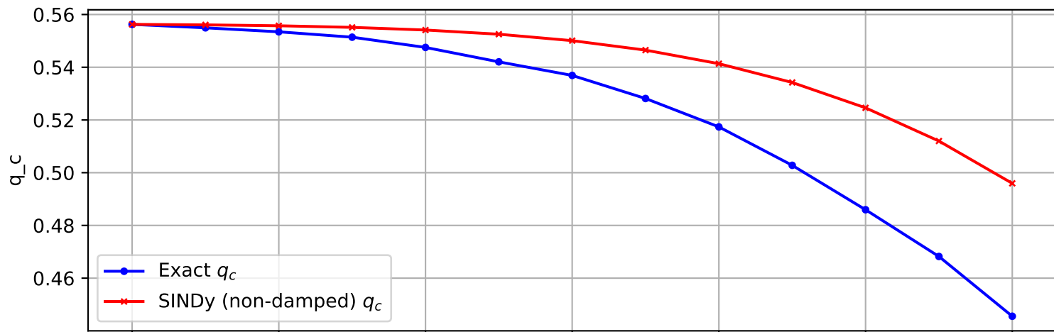
Trajectory 318 (non-damped)
