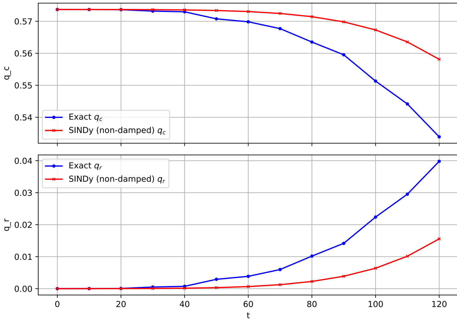
Trajectory 331 (non-damped)
