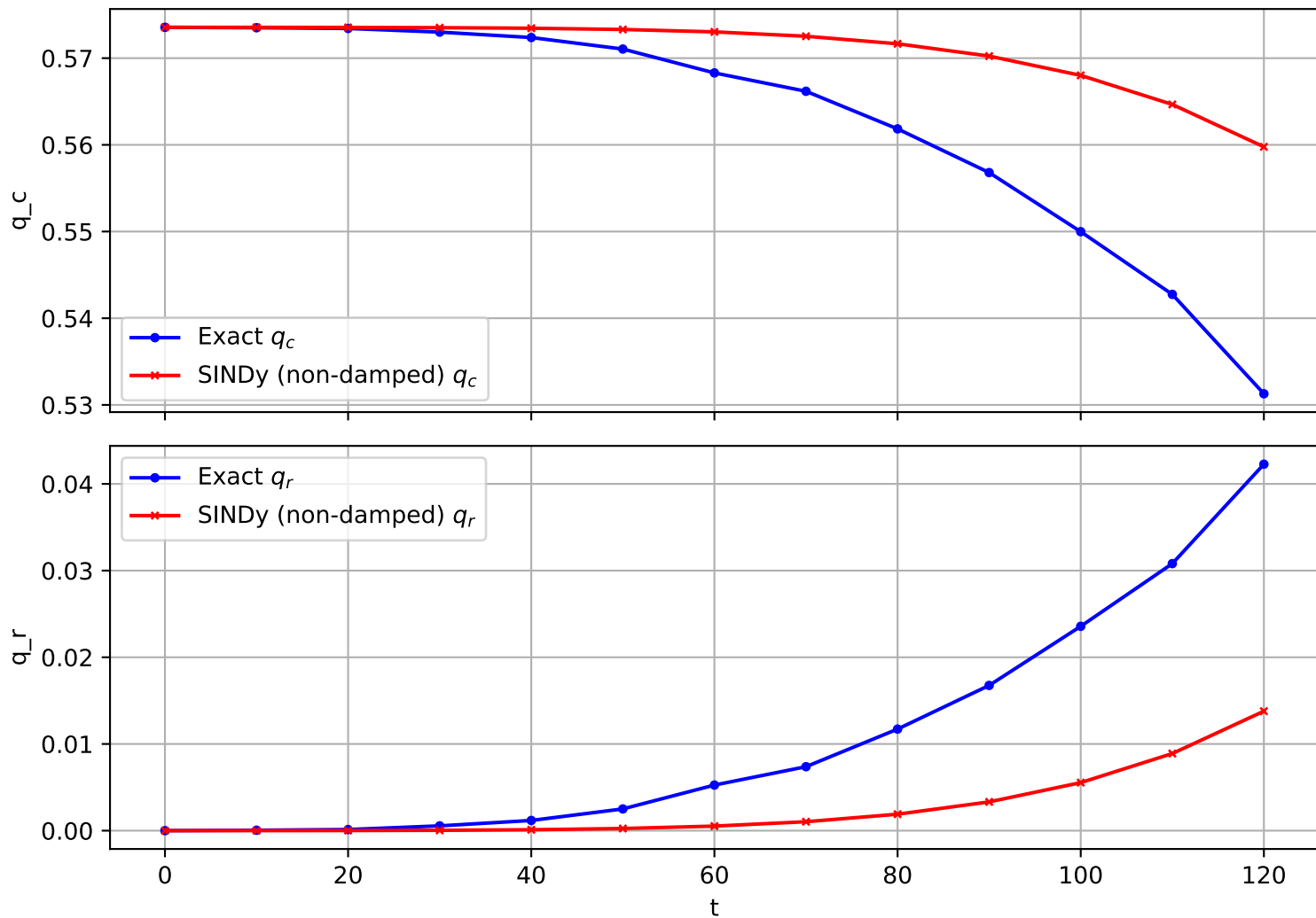
Trajectory 335 (non-damped)
