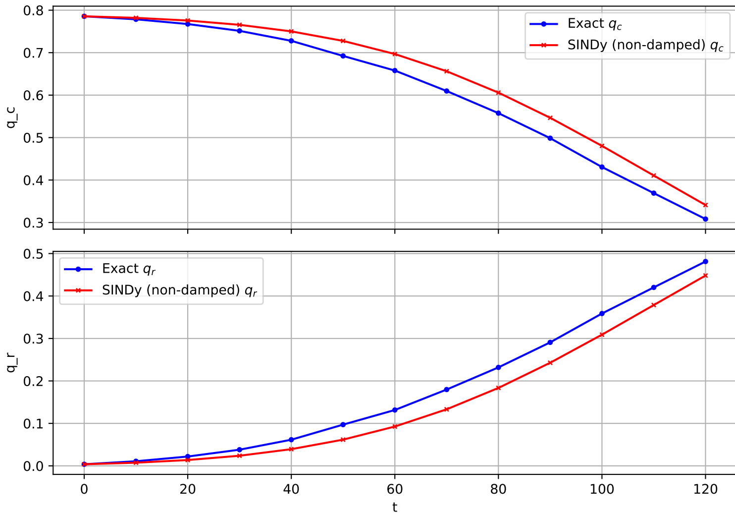
Trajectory 353 (non-damped)
