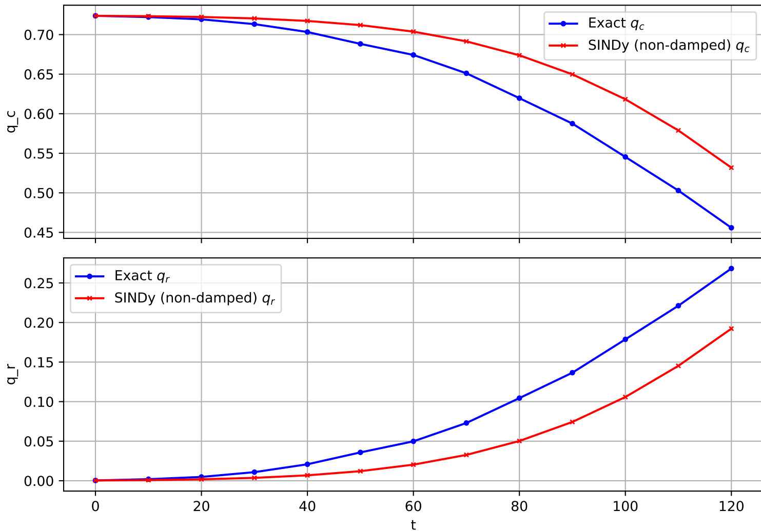
Trajectory 357 (non-damped)
