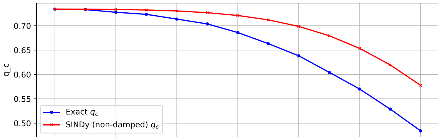
Trajectory 369 (non-damped)
