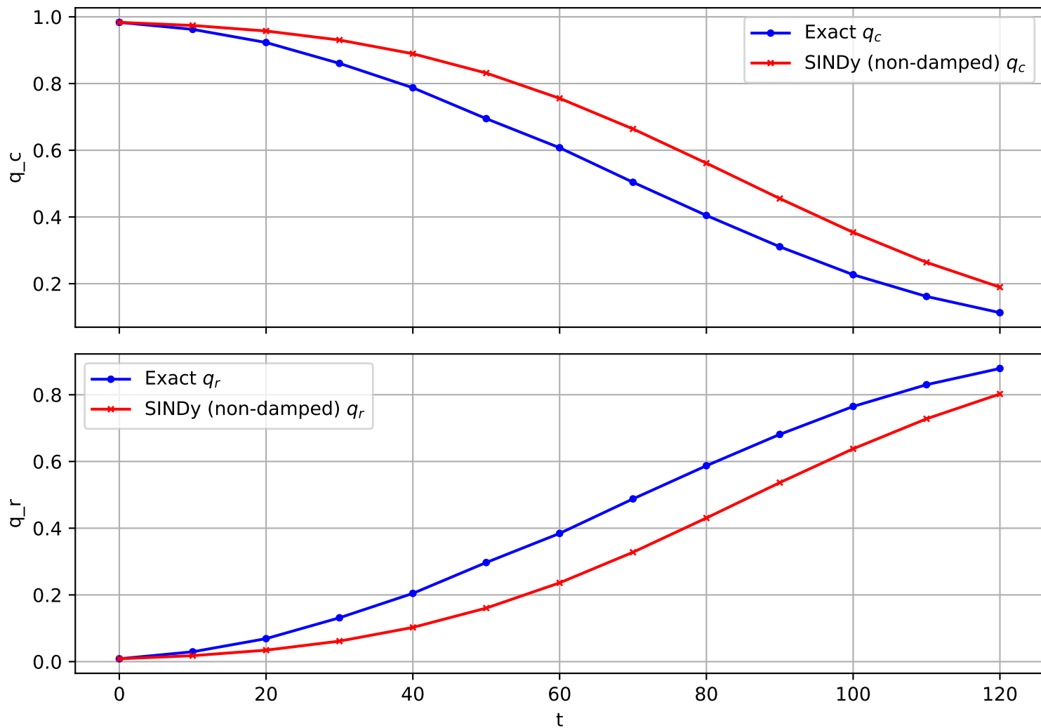
Trajectory 383 (non-damped)
