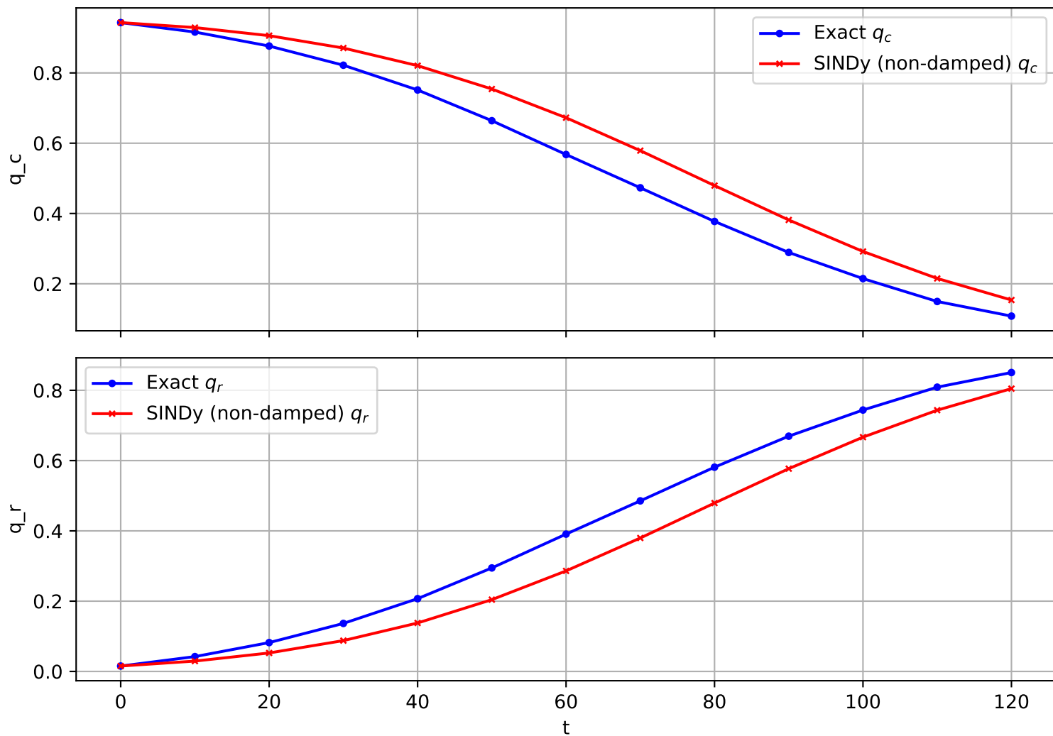
Trajectory 386 (non-damped)
