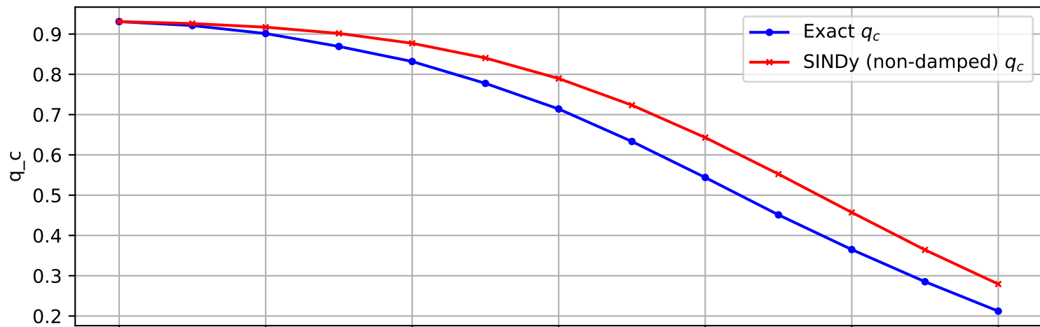
Trajectory 391 (non-damped)
