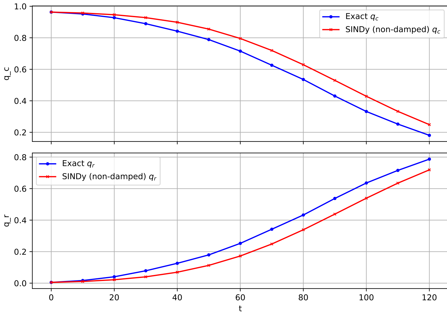
Trajectory 397 (non-damped)
