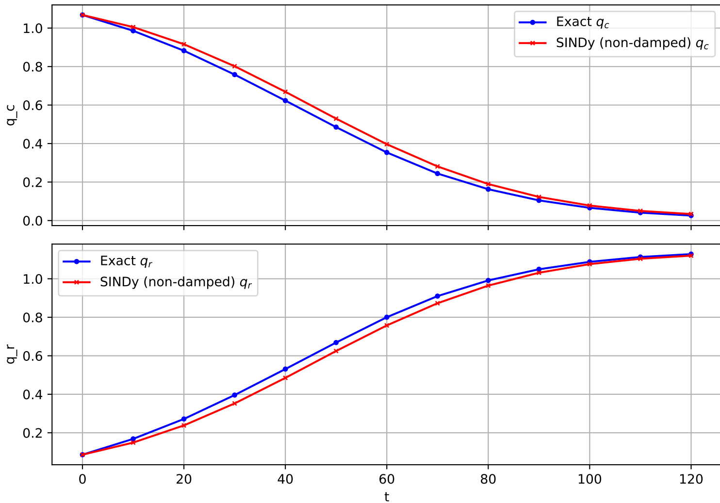
Trajectory 406 (non-damped)
