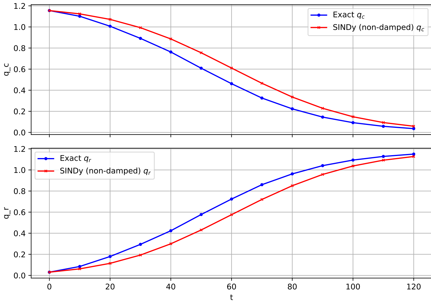
Trajectory 420 (non-damped)
