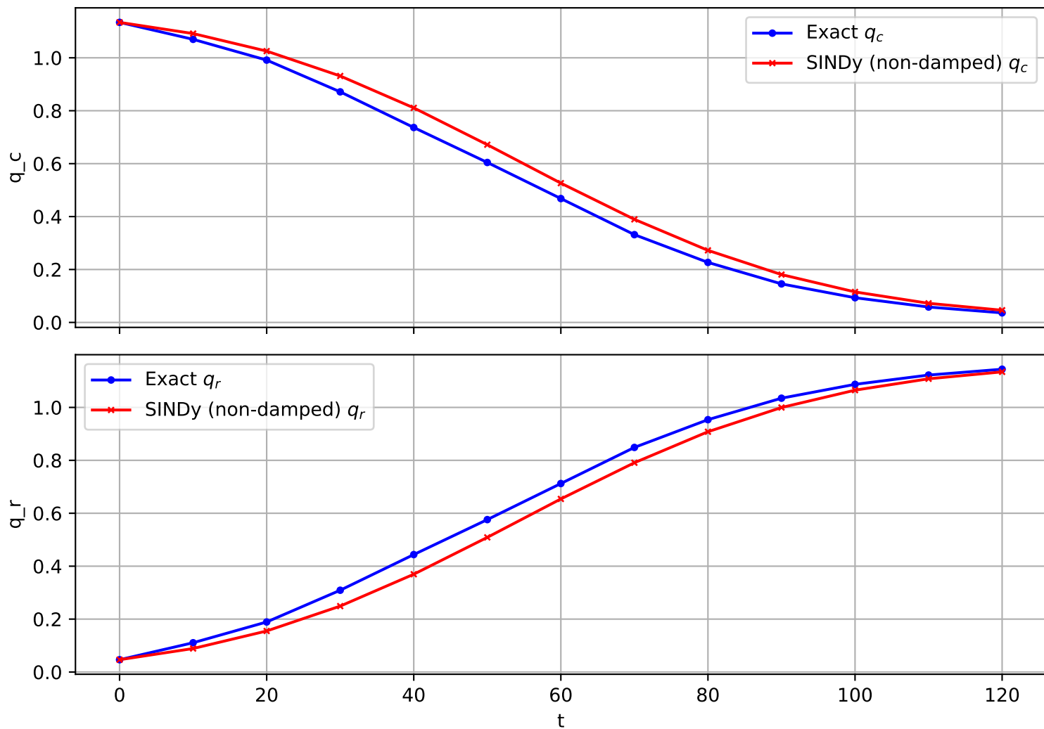
Trajectory 425 (non-damped)
