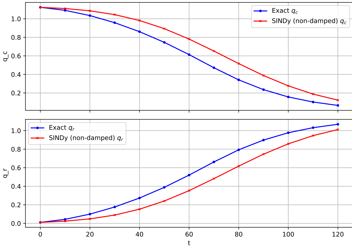
Trajectory 428 (non-damped)
