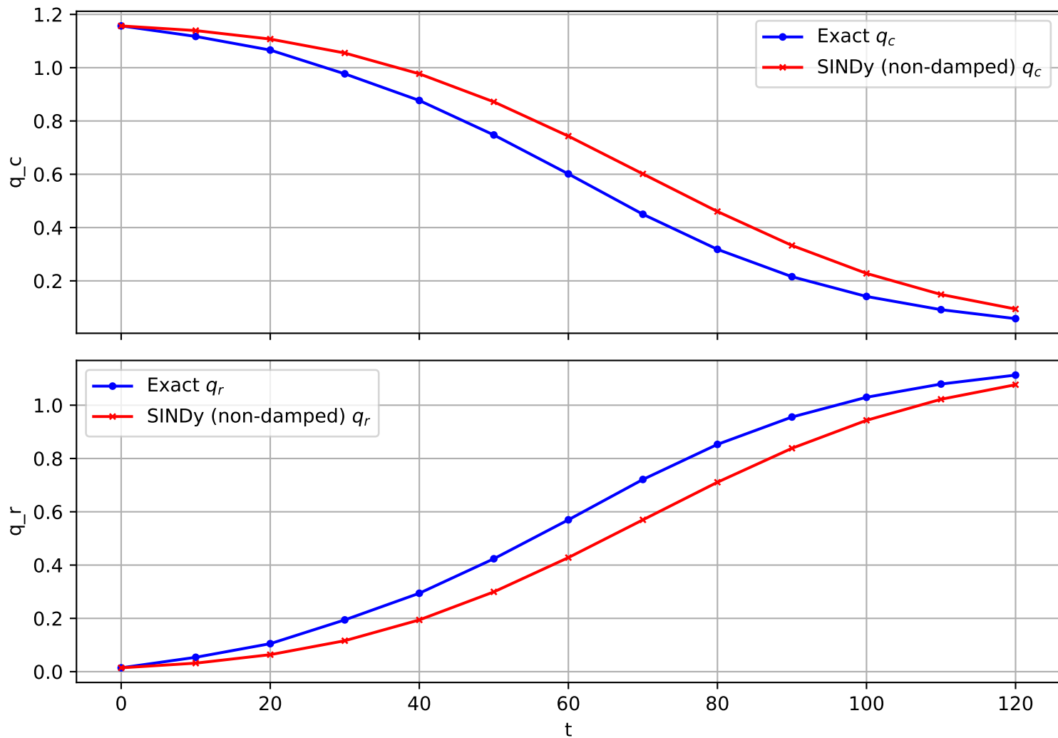
Trajectory 429 (non-damped)
