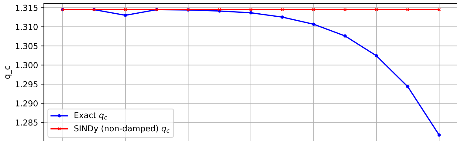
Trajectory 43 (non-damped)
