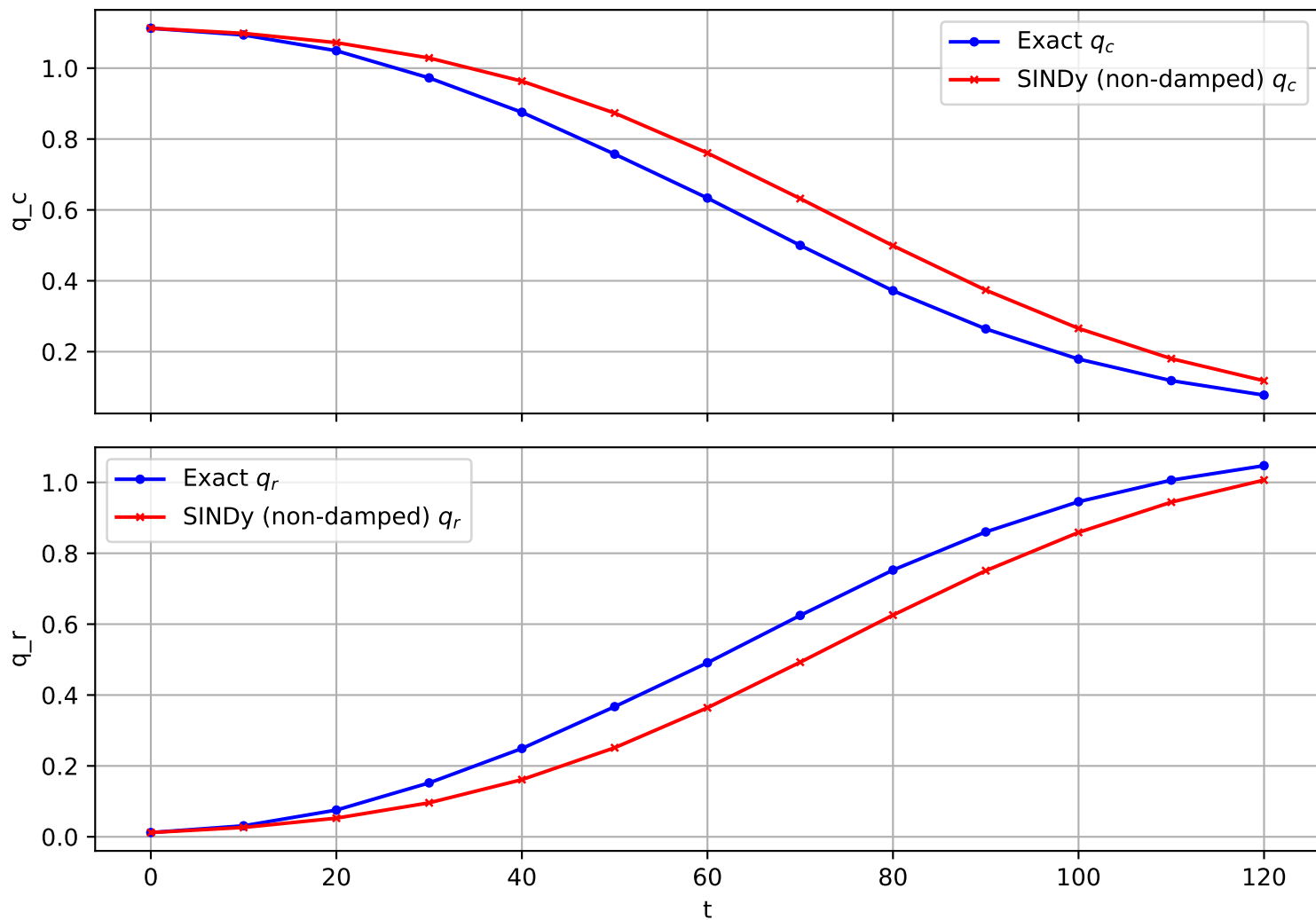
Trajectory 438 (non-damped)
