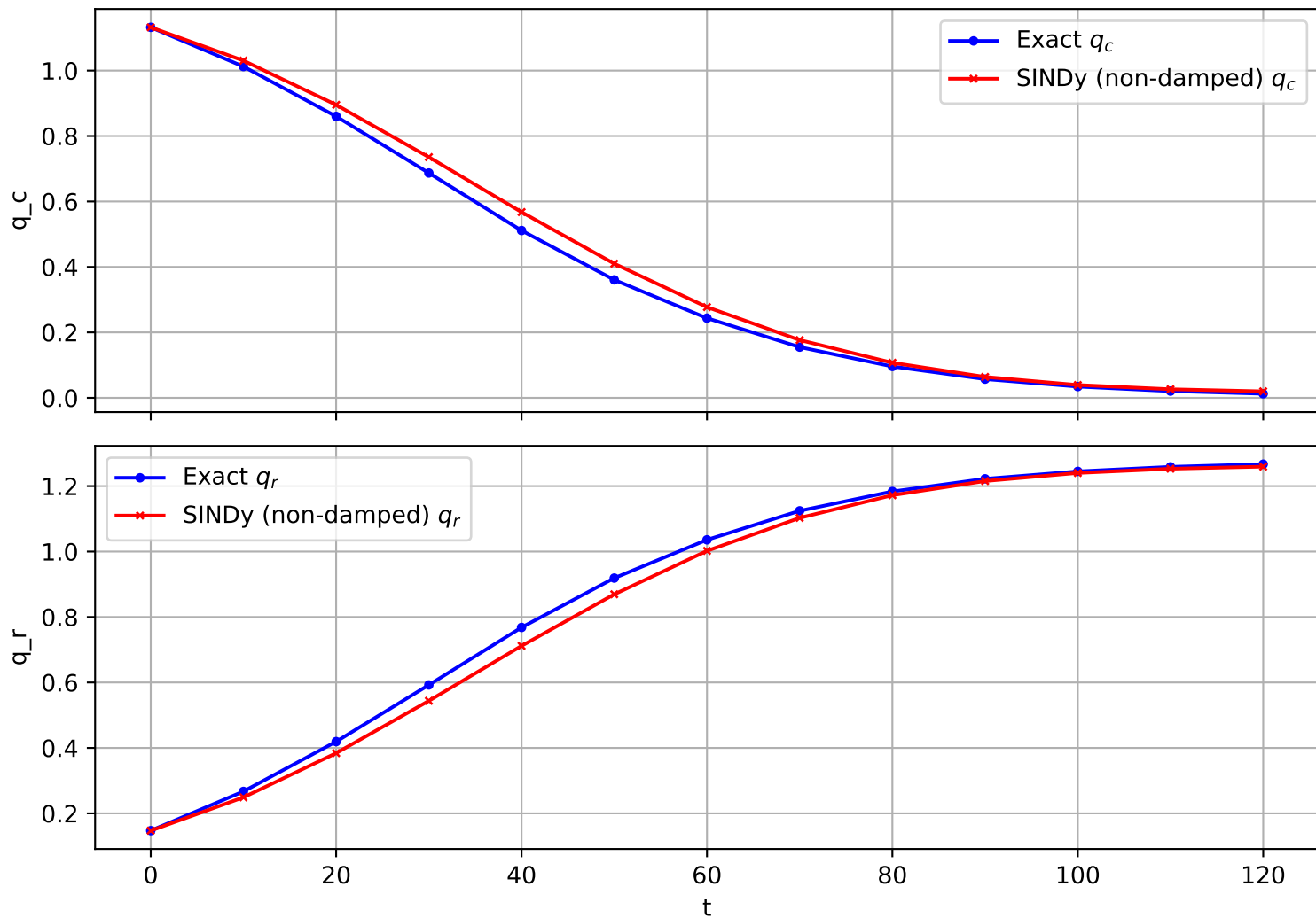
Trajectory 444 (non-damped)
