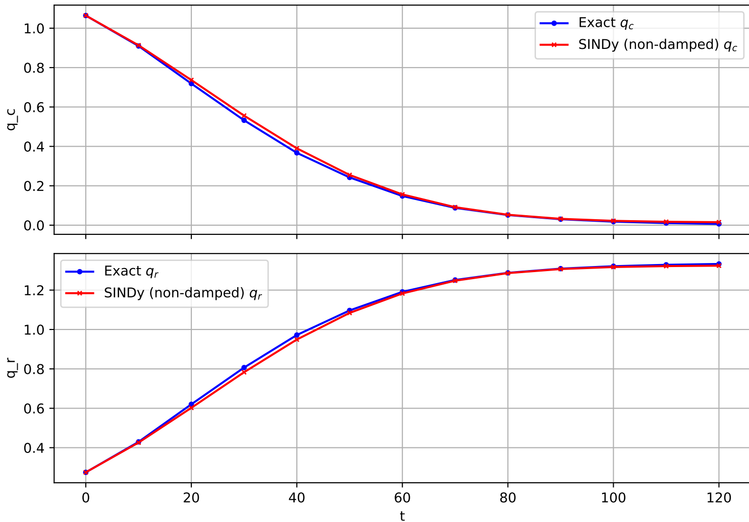
Trajectory 447 (non-damped)
