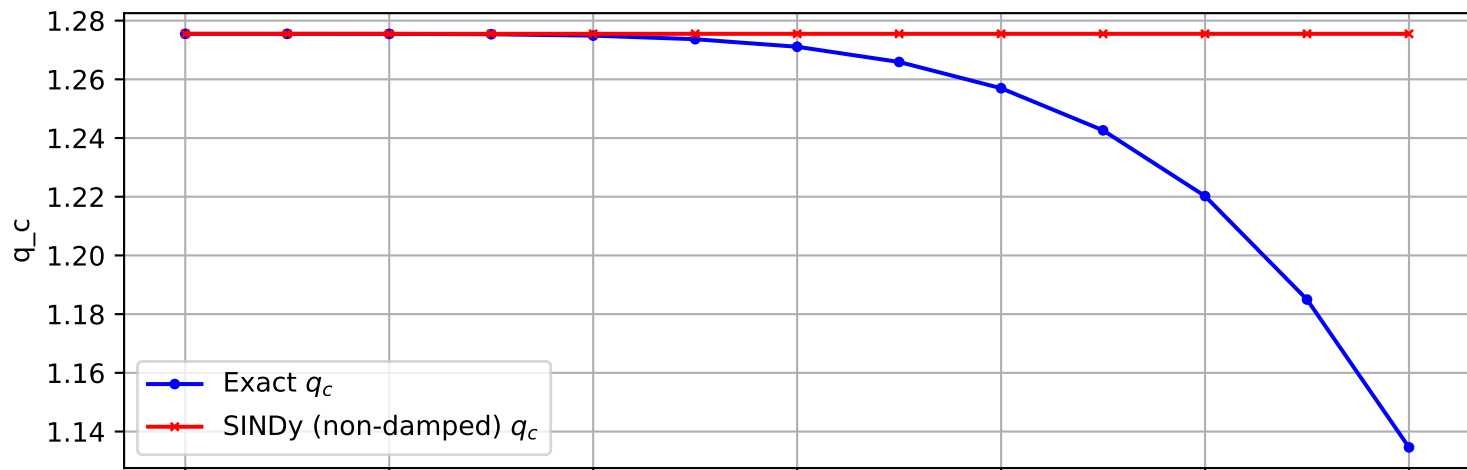
Trajectory 46 (non-damped)
