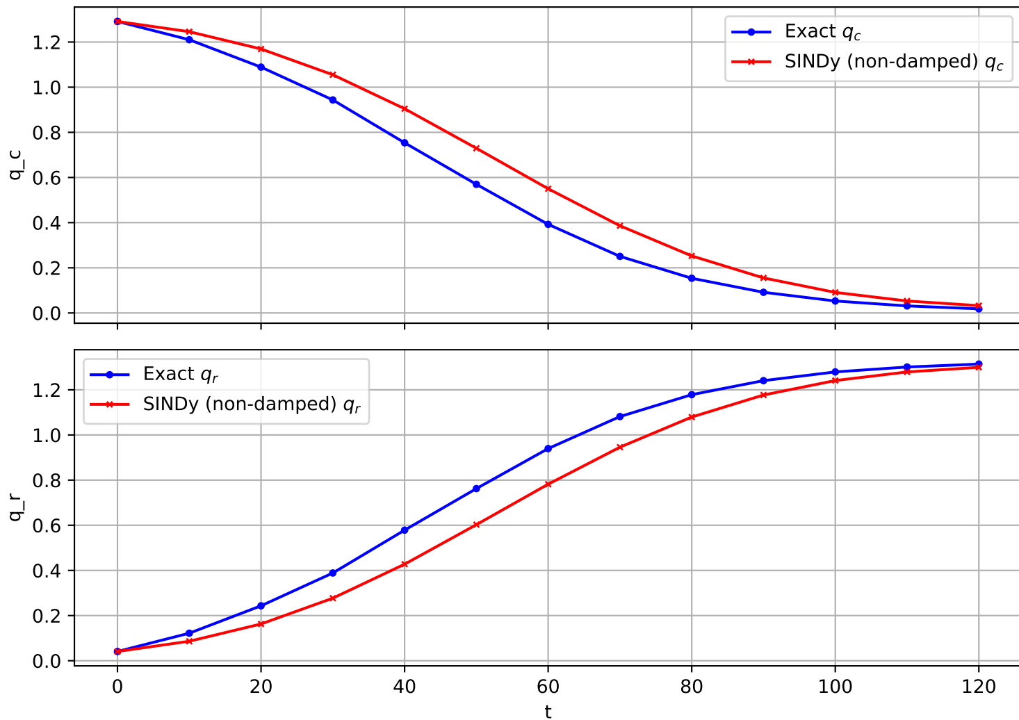
Trajectory 462 (non-damped)
