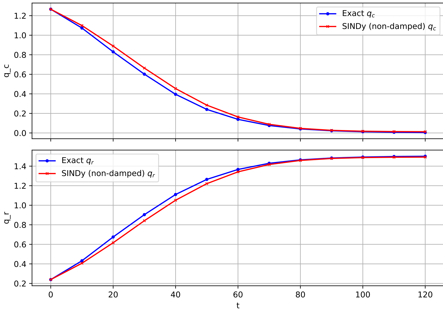
Trajectory 476 (non-damped)
