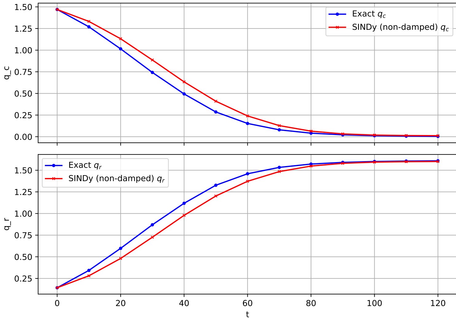
Trajectory 486 (non-damped)
