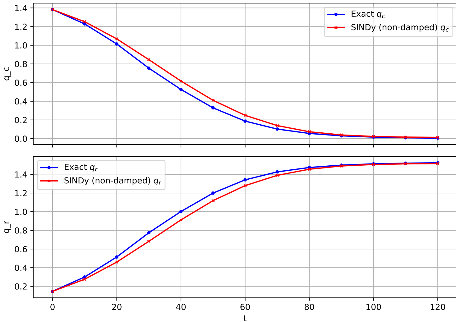
Trajectory 487 (non-damped)
