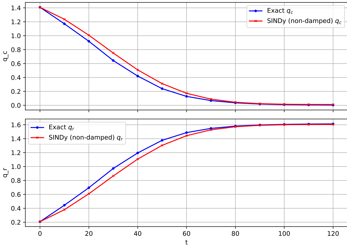
Trajectory 491 (non-damped)
