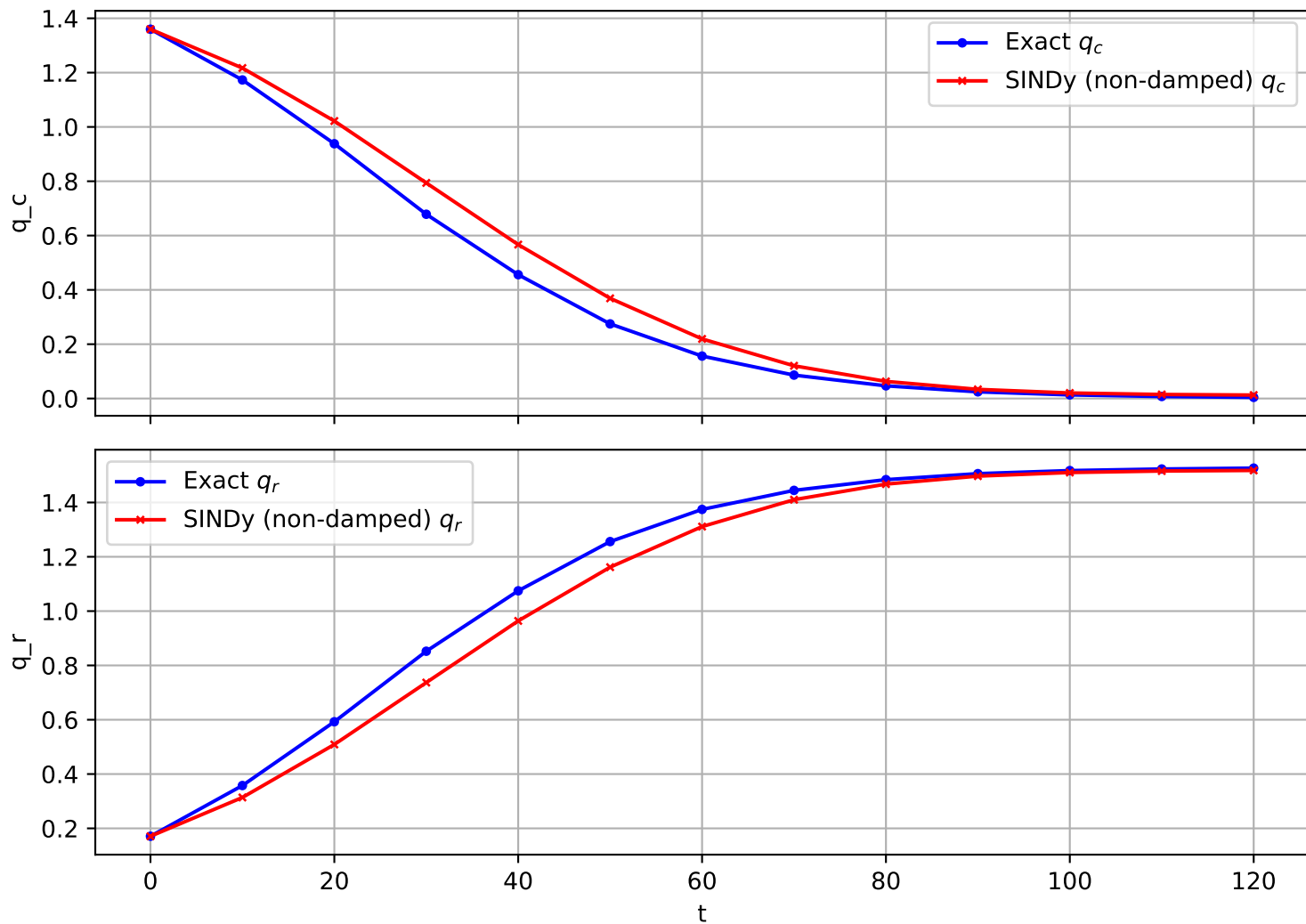
Trajectory 492 (non-damped)
