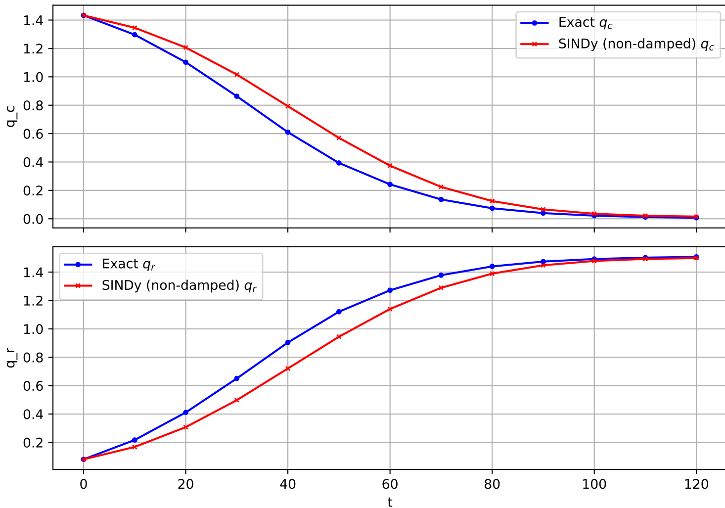
Trajectory 497 (non-damped)
