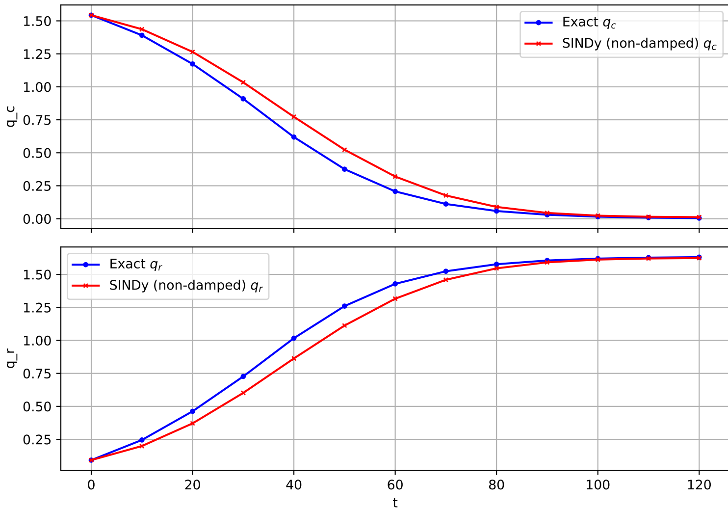
Trajectory 498 (non-damped)
