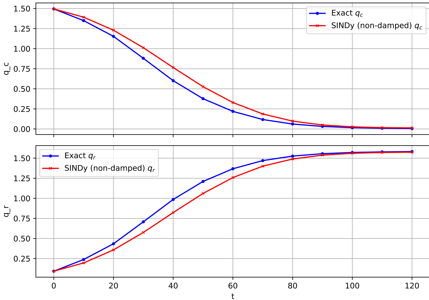
Trajectory 499 (non-damped)
