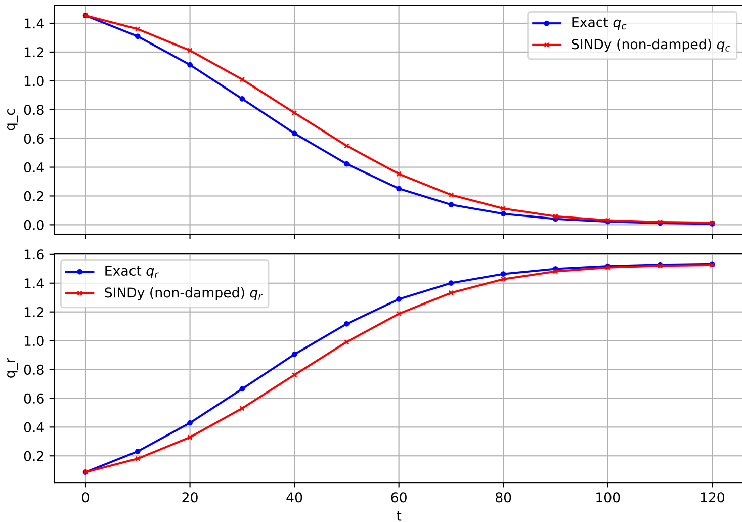
Trajectory 500 (non-damped)
