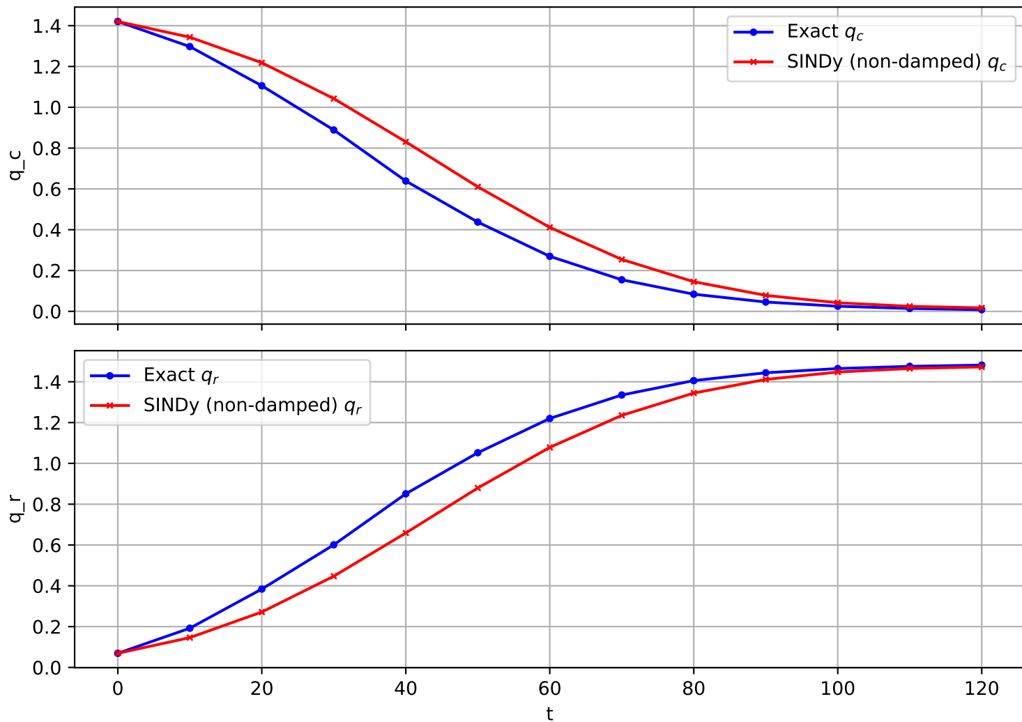
Trajectory 507 (non-damped)
