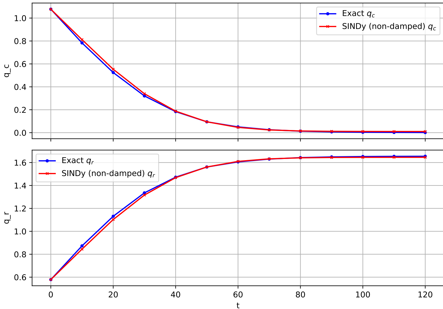
Trajectory 519 (non-damped)
