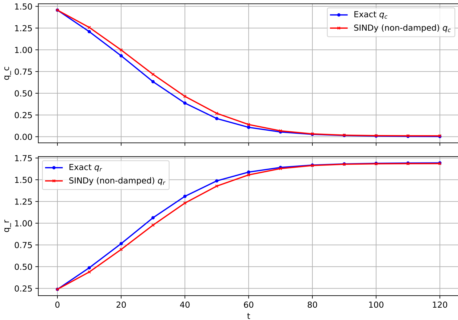
Trajectory 522 (non-damped)
