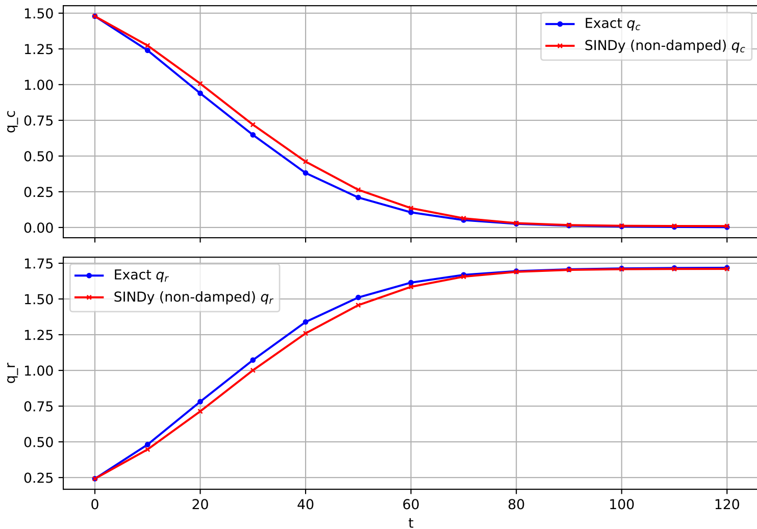
Trajectory 525 (non-damped)
