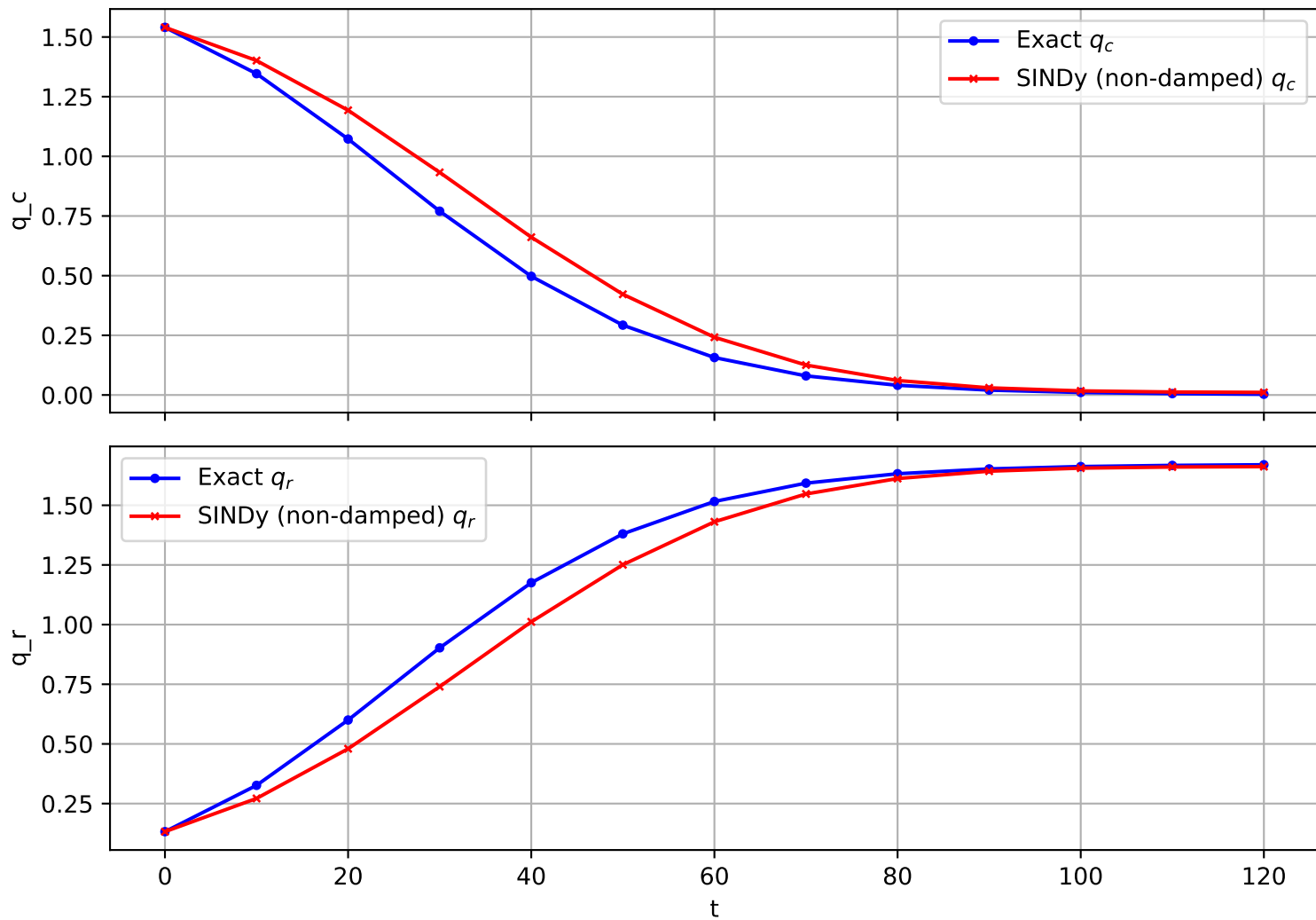
Trajectory 542 (non-damped)
