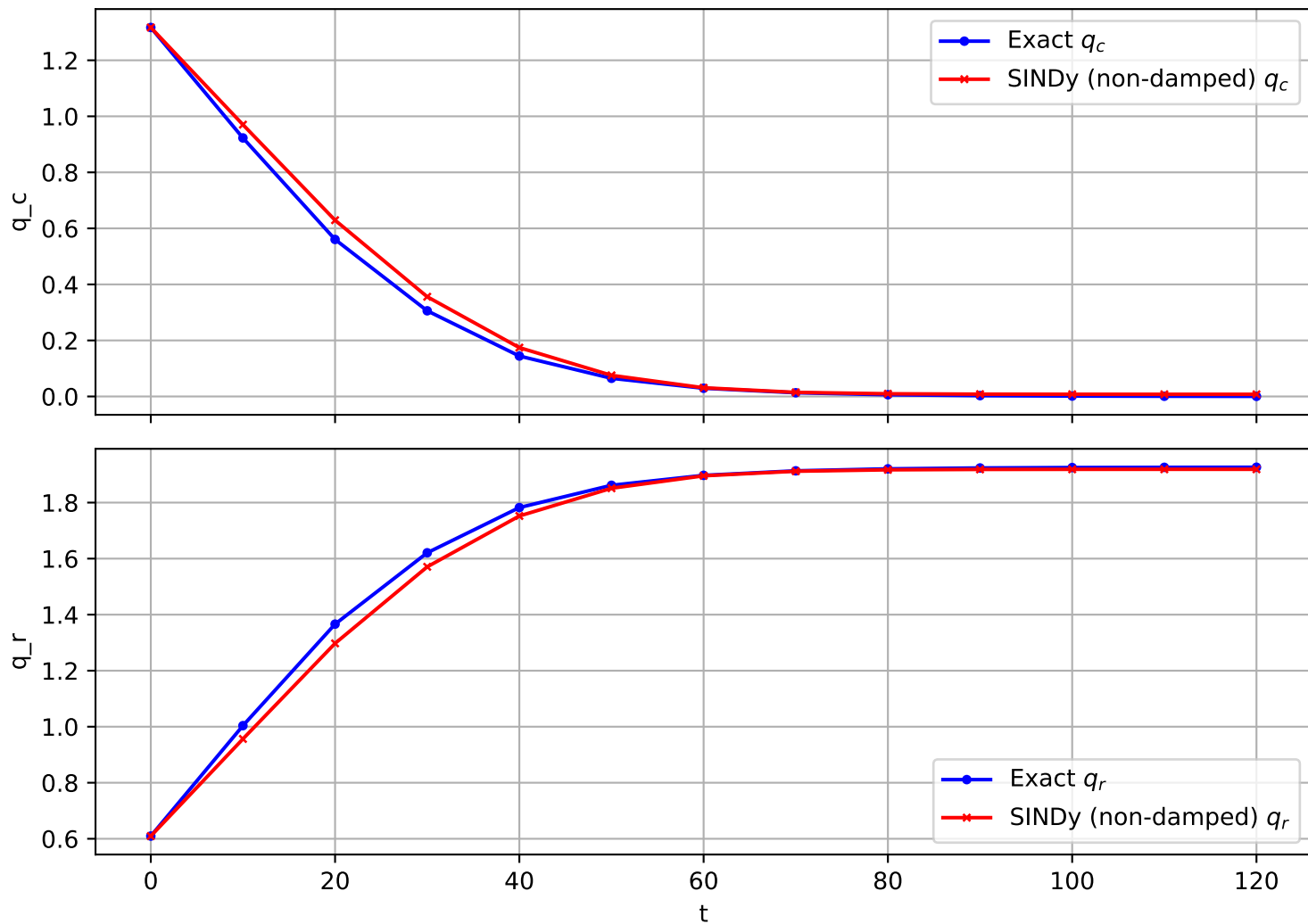
Trajectory 546 (non-damped)
