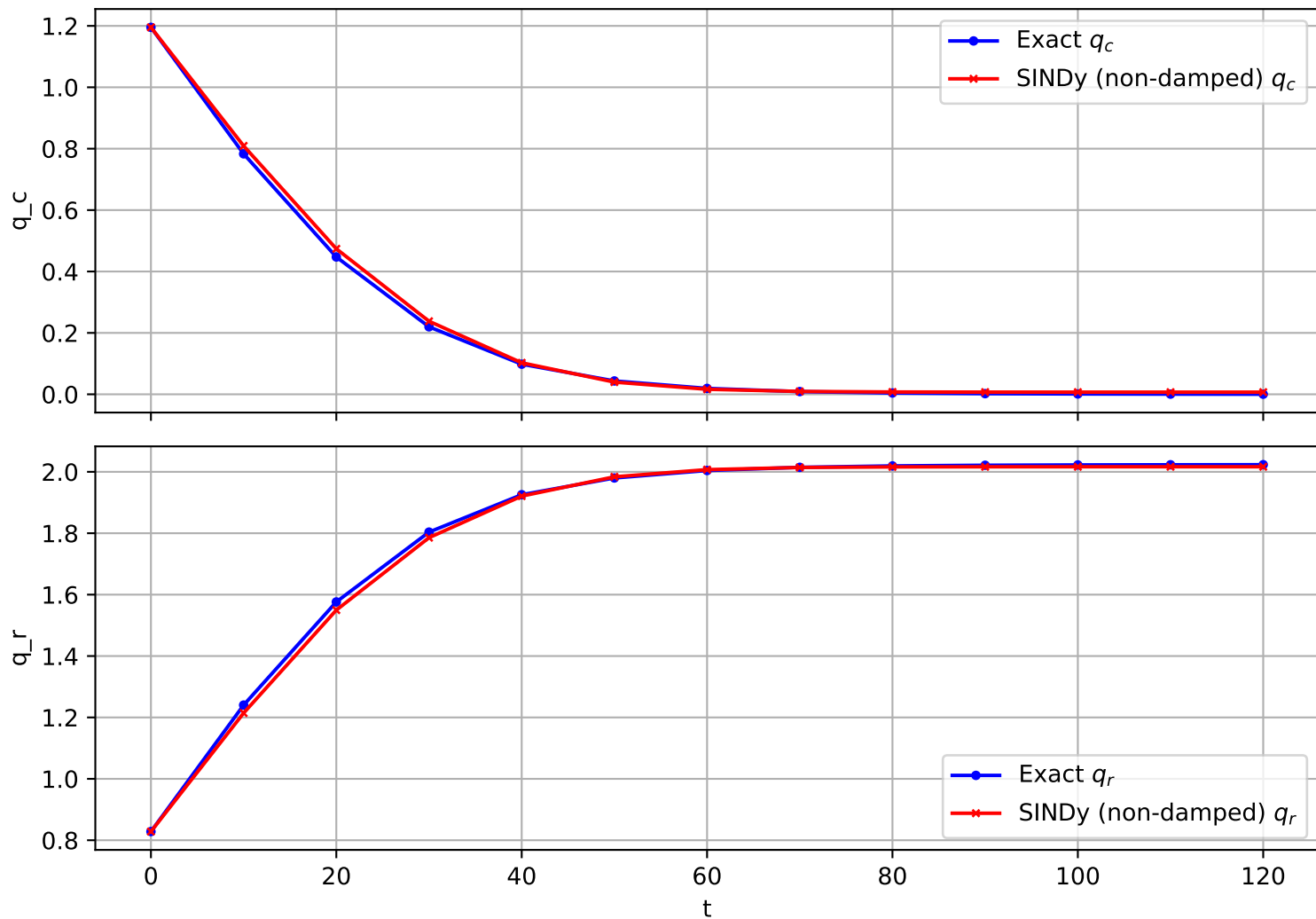
Trajectory 553 (non-damped)
