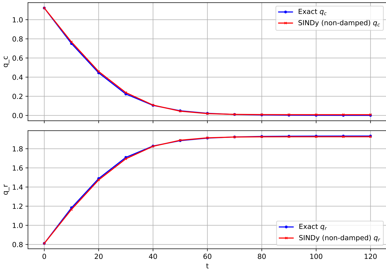
Trajectory 554 (non-damped)
