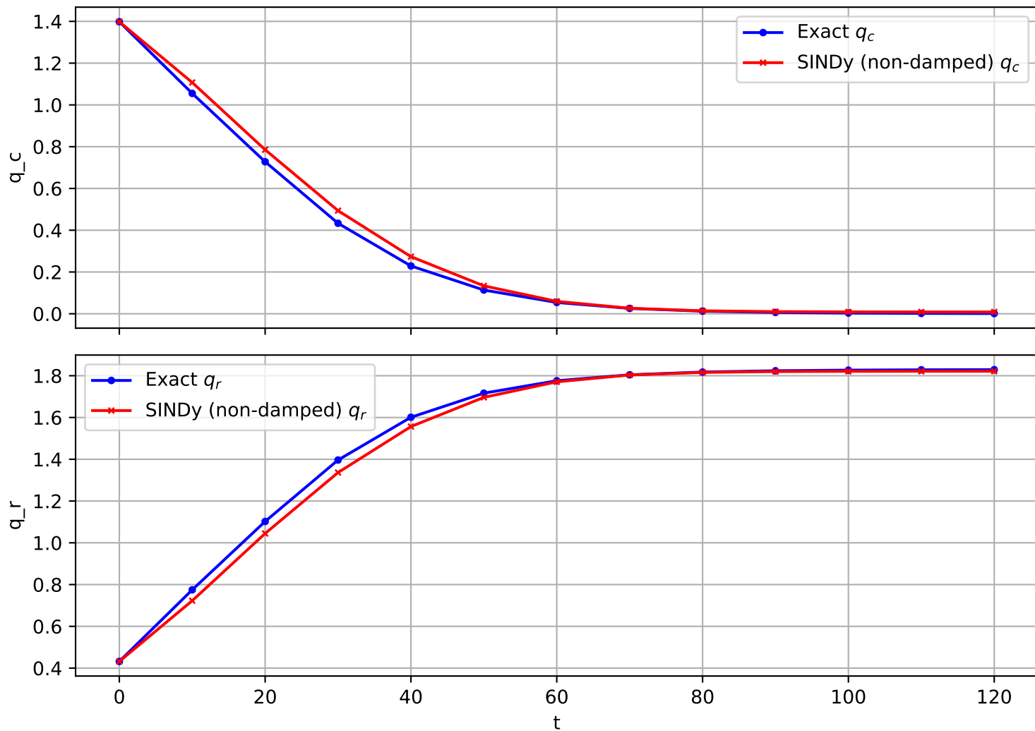
Trajectory 562 (non-damped)
