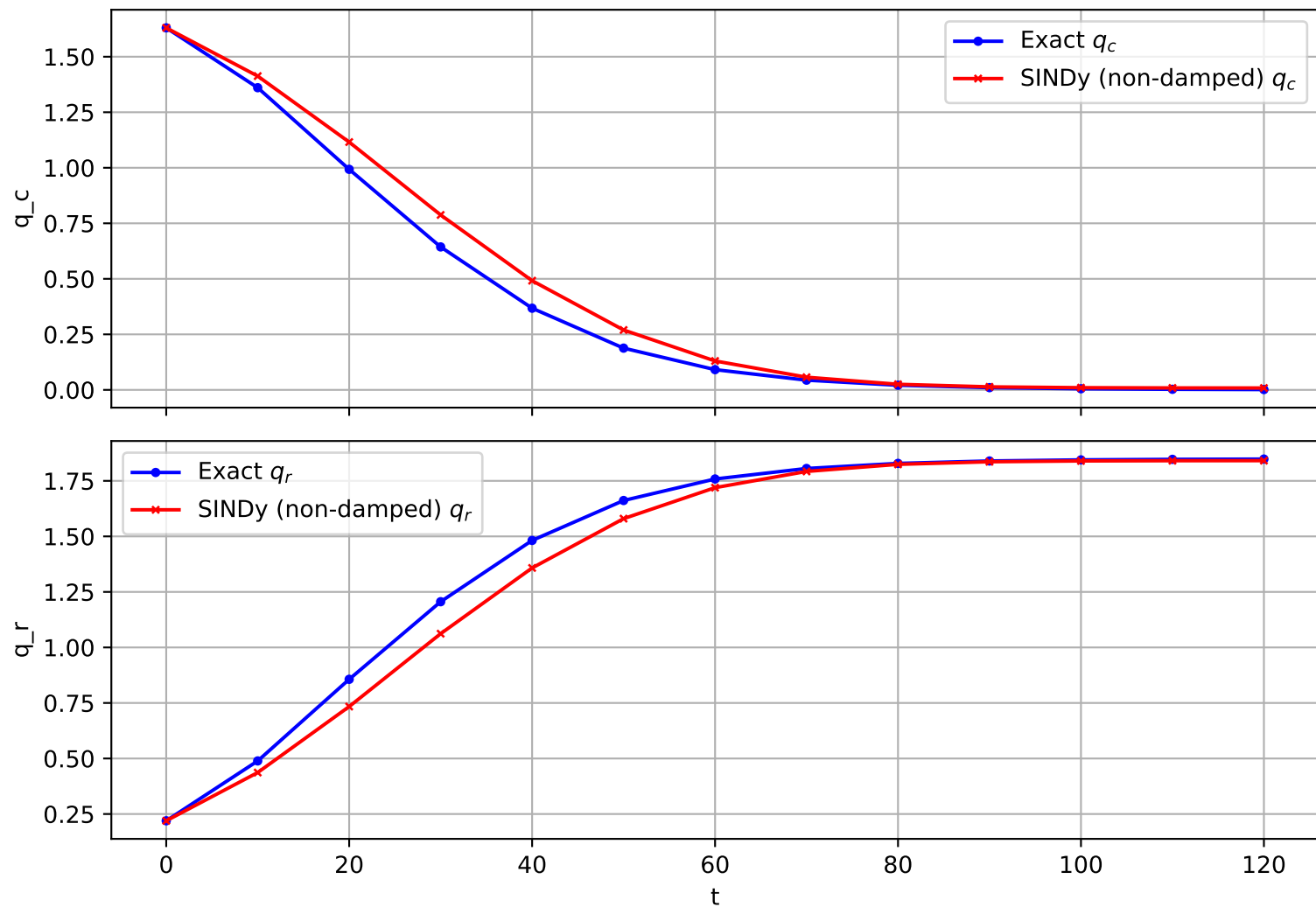
Trajectory 576 (non-damped)
