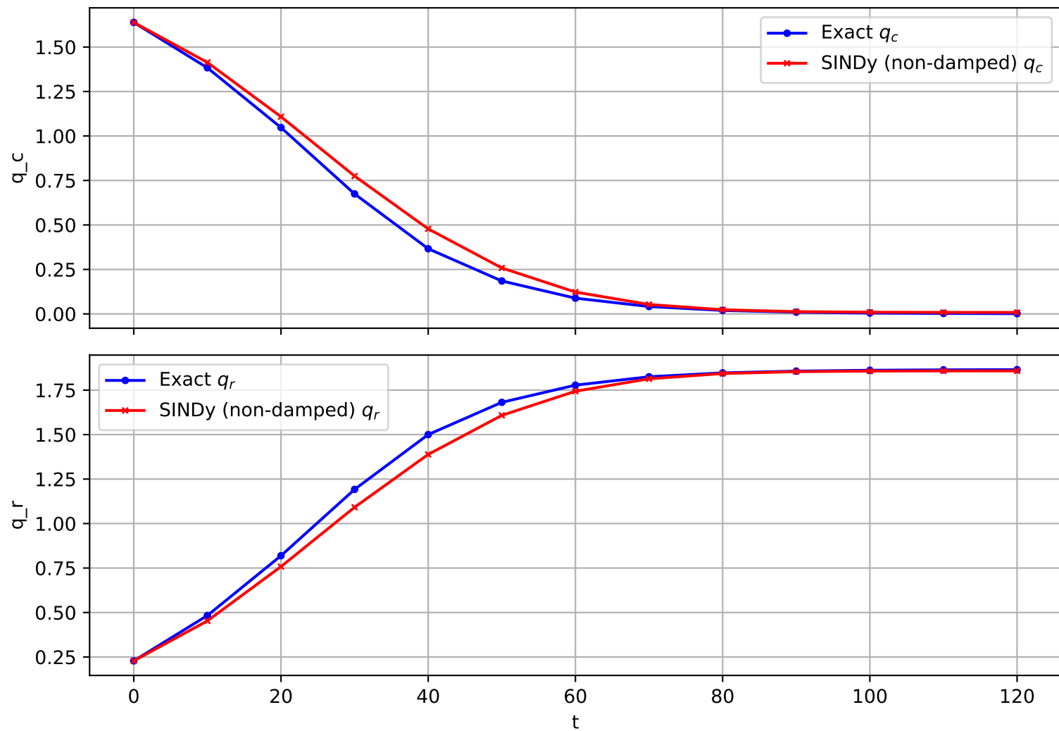
Trajectory 579 (non-damped)
