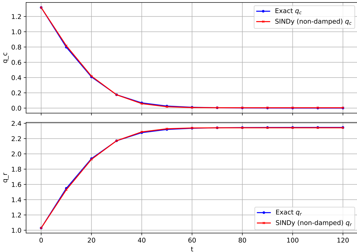
Trajectory 585 (non-damped)
