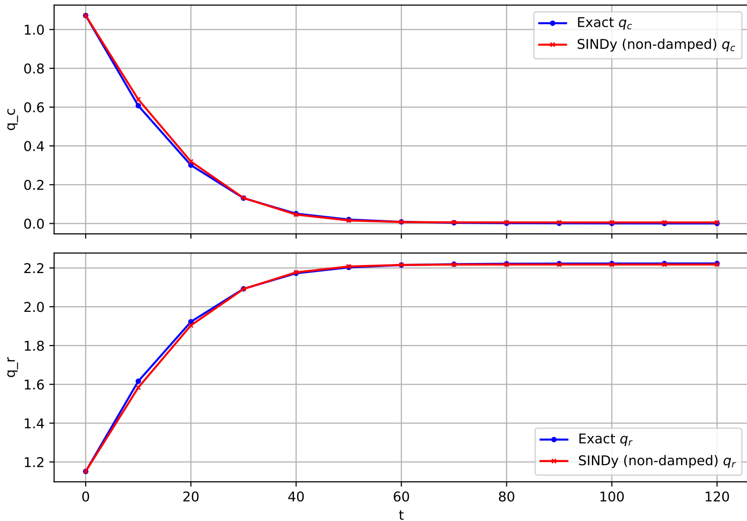
Trajectory 587 (non-damped)
