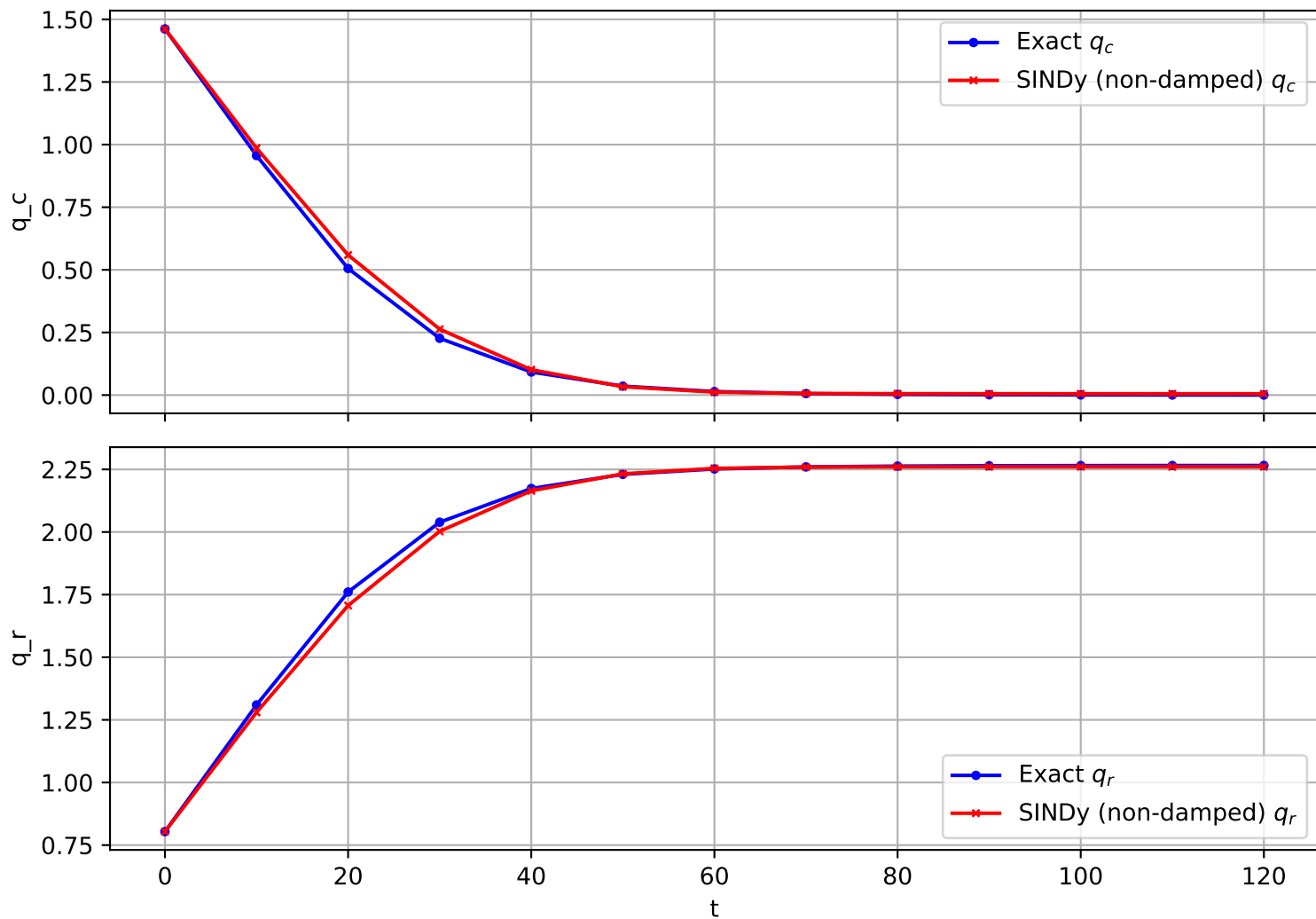
Trajectory 600 (non-damped)
