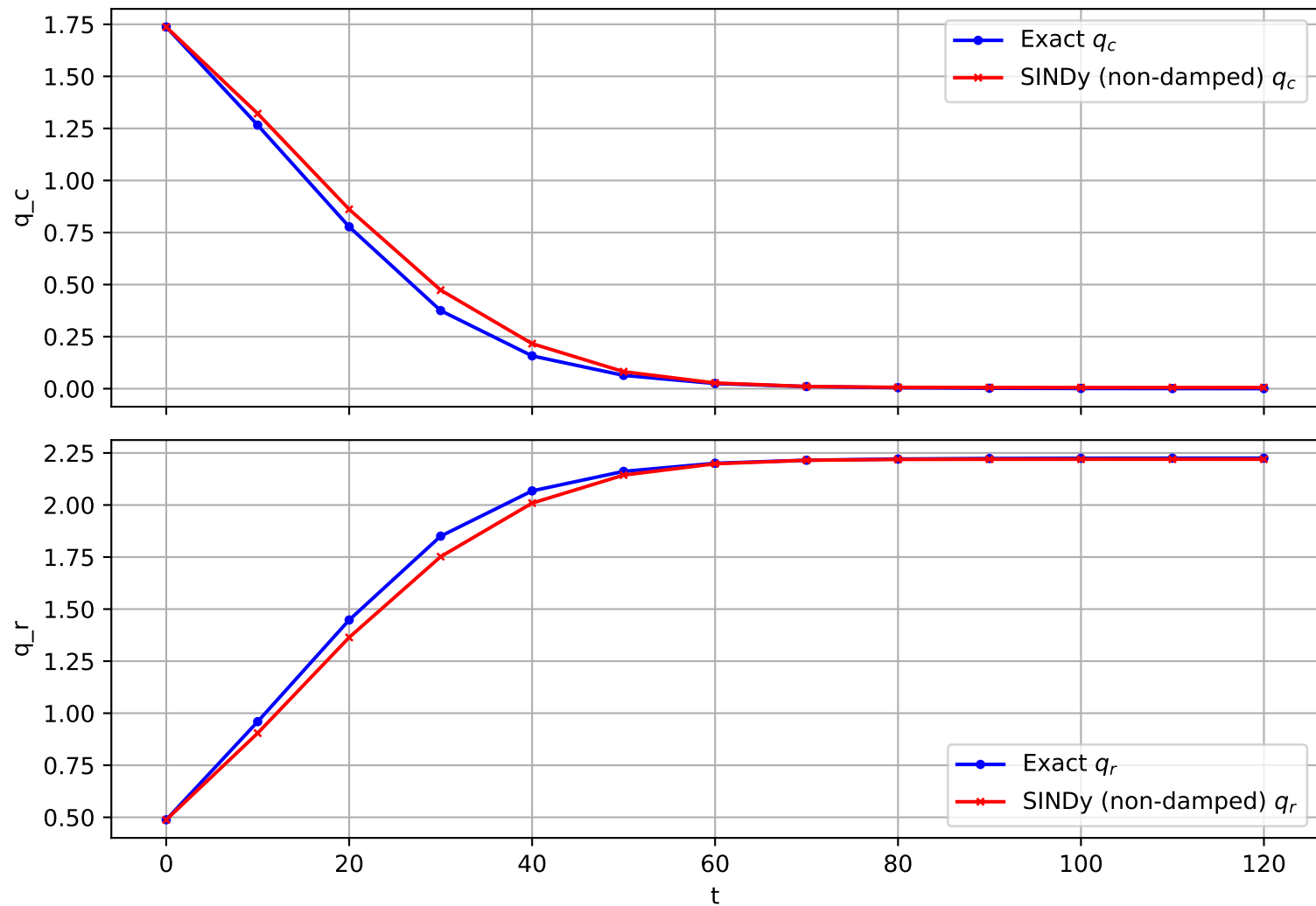
Trajectory 612 (non-damped)
