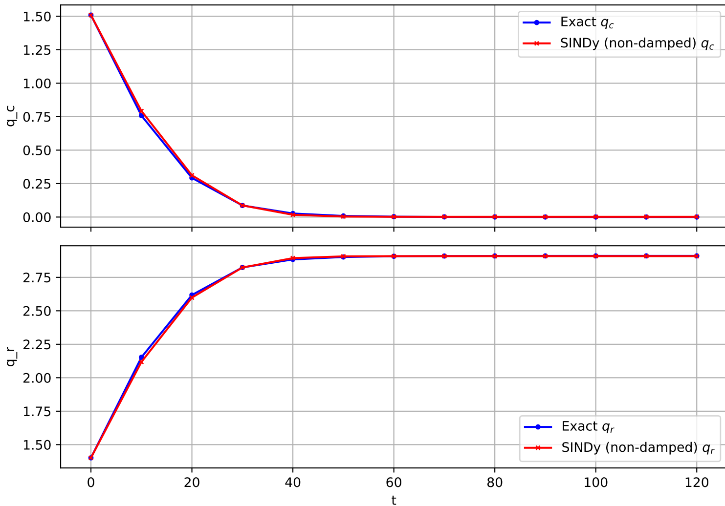
Trajectory 627 (non-damped)
