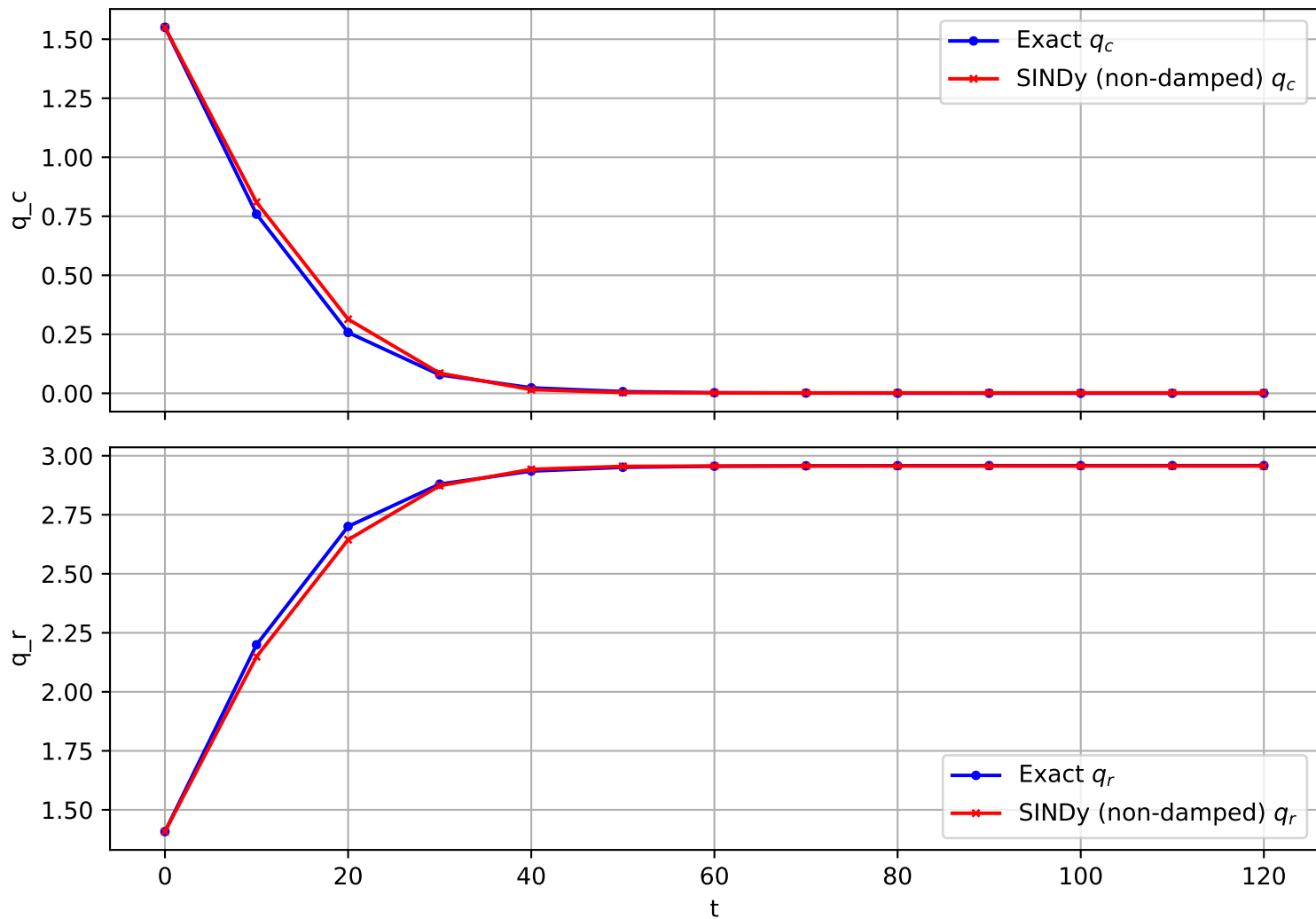
Trajectory 630 (non-damped)
