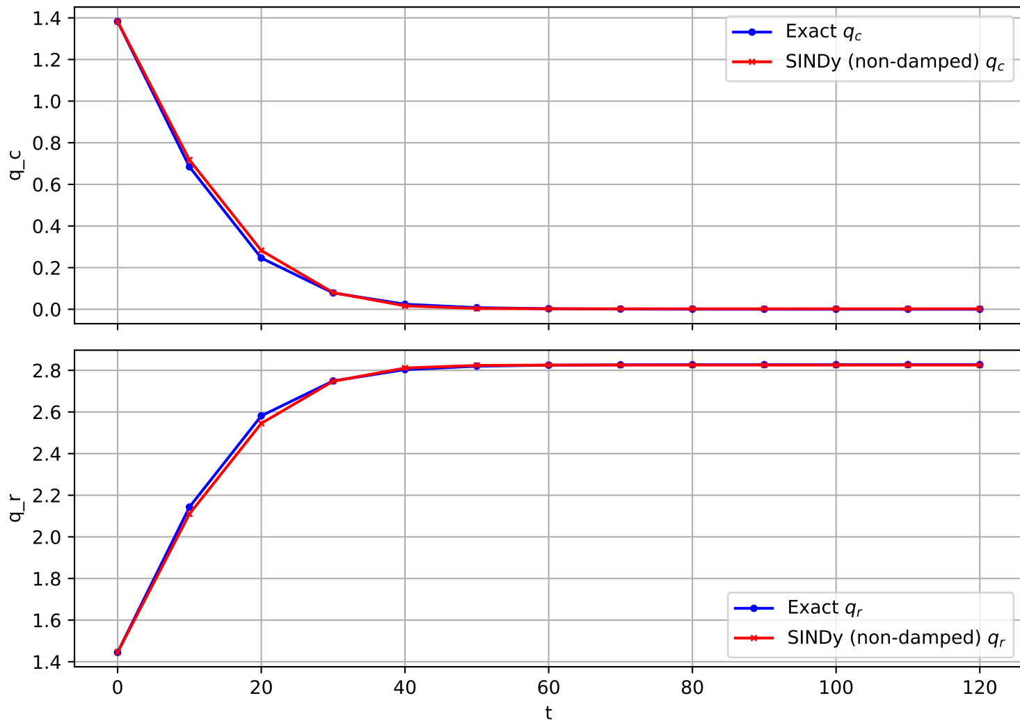
Trajectory 633 (non-damped)
